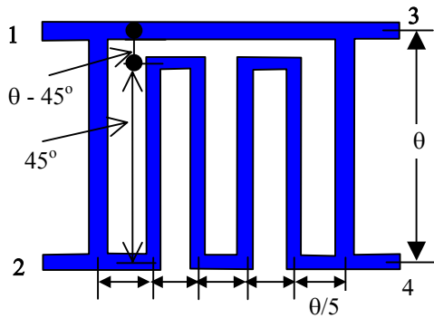
Fig. 5 Layout of square shape coupler
