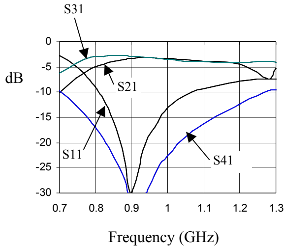
Fig.10 Experimental results of the coupler layout shown in Fig.4
