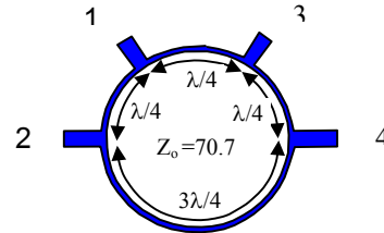
Fig. 1 Layout of the conventional ring coupler based on \lambda_g/4 line
