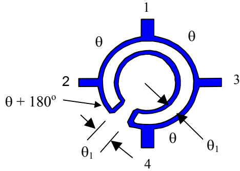
Fig. 4 Layout of small size ring coupler for symmetrical feeding ports
