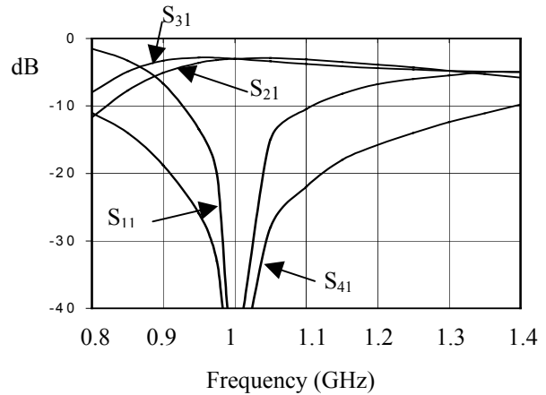
Fig. 8 Simulation results based on ideal transmission line performed using Puff software for narrow band case
