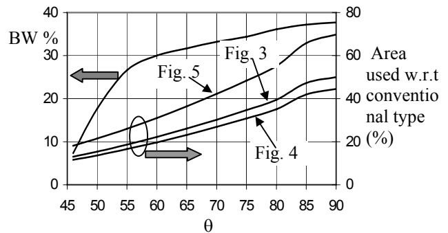
Fig. 6: Relative bandwidth and percentage area used w.r.t. the conventional coupler of Figs.3-5
