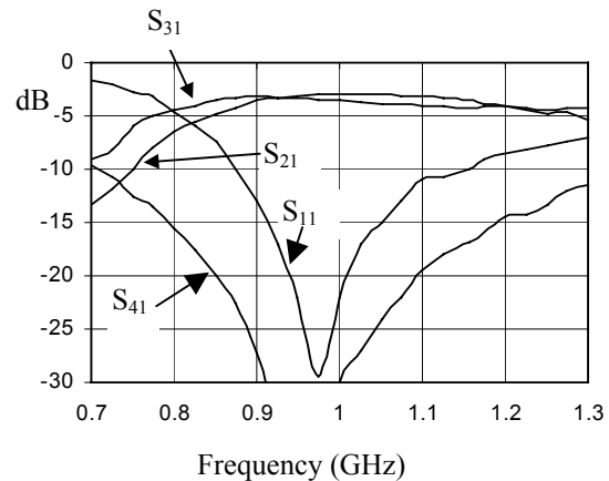
Fig. 9 Simulation results, performed by IE3D, of the layout of the circuit in Fig.4
