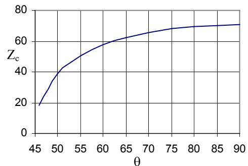
Fig. 7 Arms characteristic impedance Z_c against arms electrical length \theta
