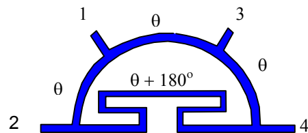
Fig. 3 Layout of small size ring coupler for asymmetrical feeding ports
