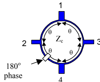
Fig. 2 Layout of a small size ring coupler derived from the theory in [4]
